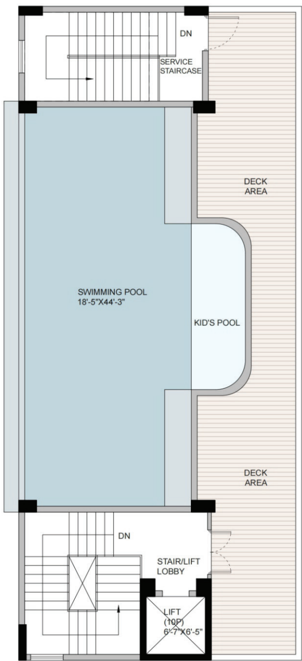
ROOF TOP PLAN
